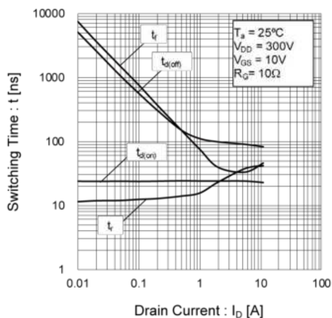
Fig.15 Switching Characteristics
