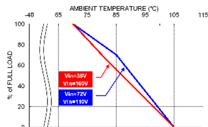
RCD15-110S00W Derating Curve
