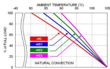
RCD15-24S05W Derating Curve With Heat-sink
