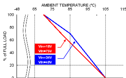
RCD15-48S00W Derating Curve
