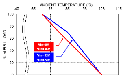
RCD15-24S00W Derating Curve
