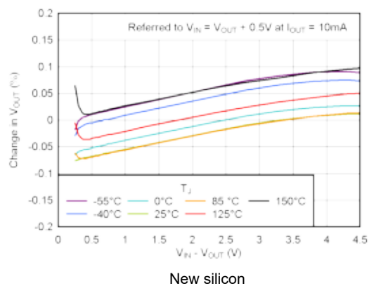
Figure 5-4. Line Regulation
