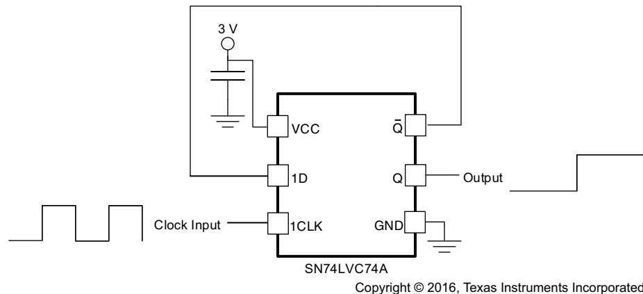
Figure 8-1. Frequency Divider
