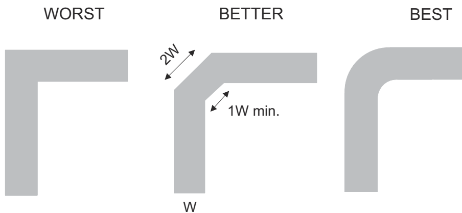
Figure 8-3. Trace Example
