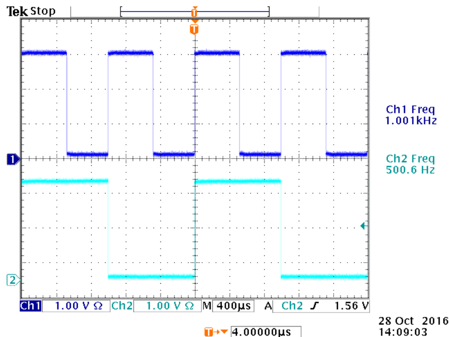
Figure 8-2. Frequency Division
