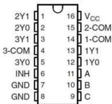
Figure 4-1. SN74LV4053A D, PW or DYY Packages, 16-Pin SOIC, TSSOP or SOT-23-THIN (Top View)
