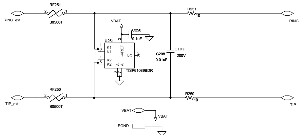
Figure 14. Flyback Protection 2
