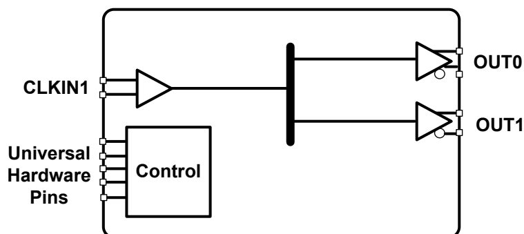
Figure 3.5. Si53352BDxxxxx-AM Functional Block Diagram
