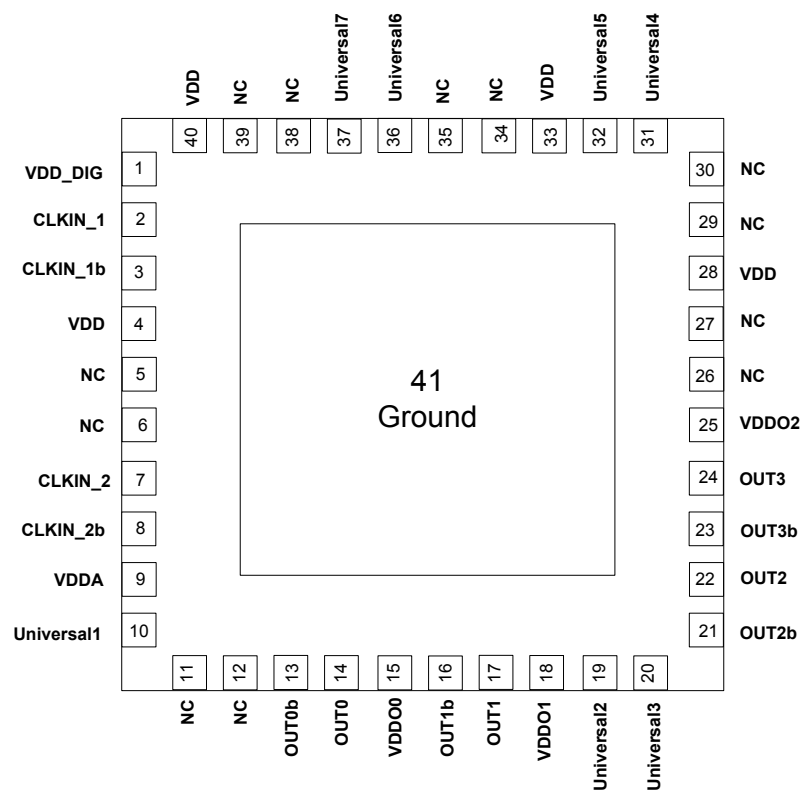
Figure 6.6. Si53354BDxxxxx-AM 40-QFN
