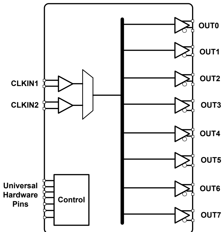
Figure 3.7. Si53358BDxxxxx-AM Functional Block Diagram
