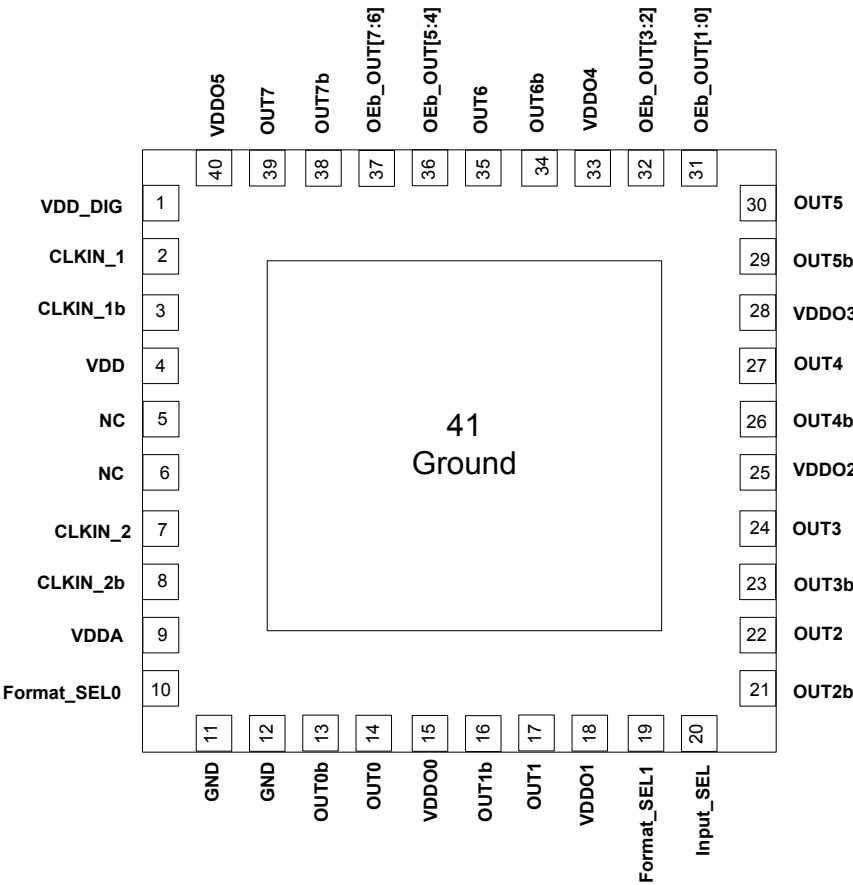
Figure 6.3. Si53358A-D01AM and Si53352BD12749-AM (40-QFN)
