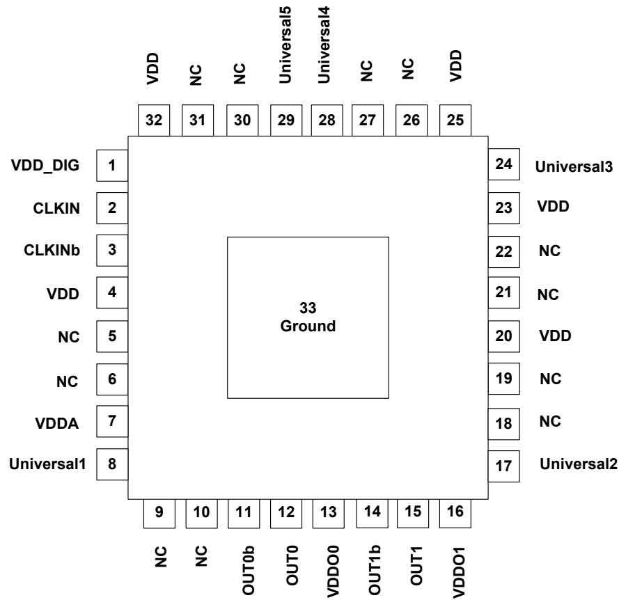
Figure 6.8. Si53352A-Dxxxxx-AM 32-QFN
