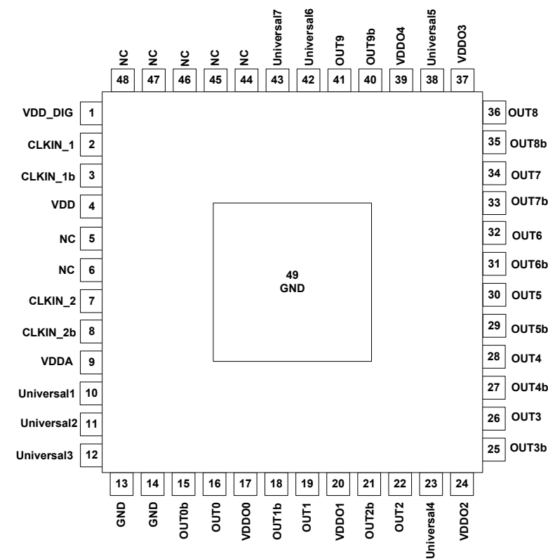
Figure 6.2. Si53350BDxxxxx-AM 48-QFN
