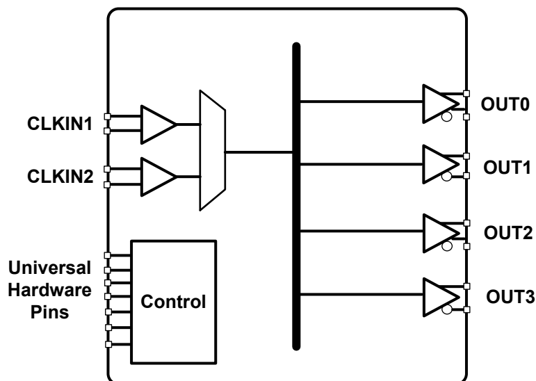
Figure 3.6. Si53354BDxxxxx-AM Functional Block Diagram
