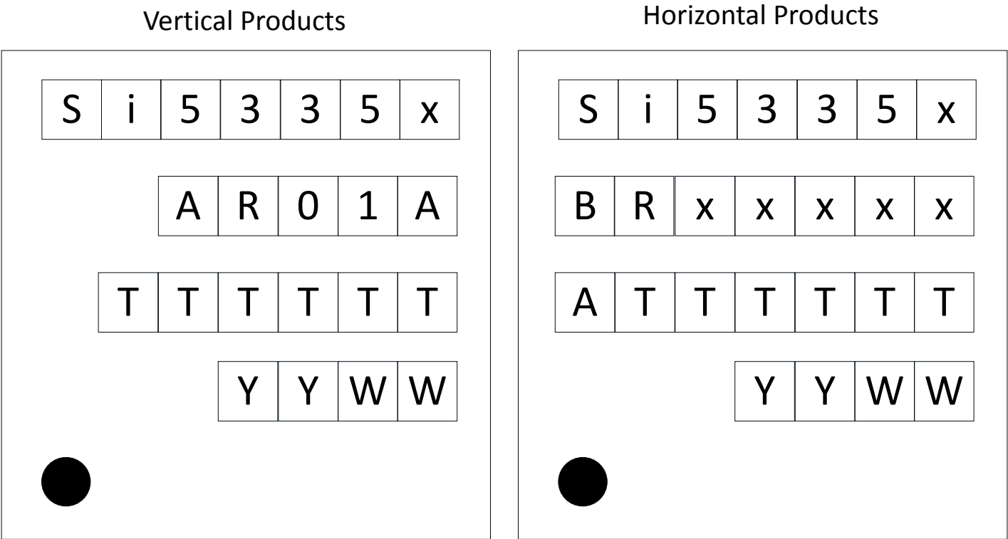
Figure 9.1. Top Marking
