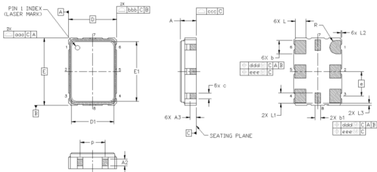
Figure 6.1. Si569 (5x7 mm) Outline Diagram
