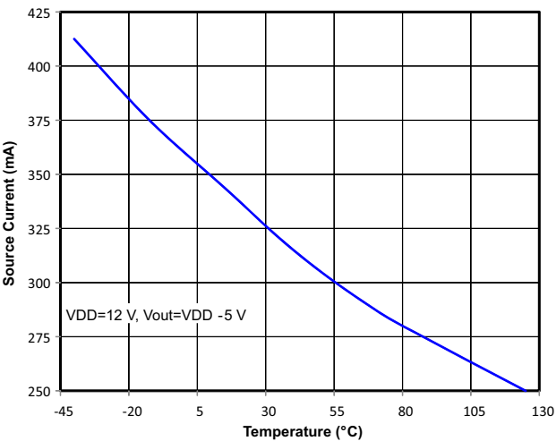
Figure 15. Output Source Current vs. Temperature
