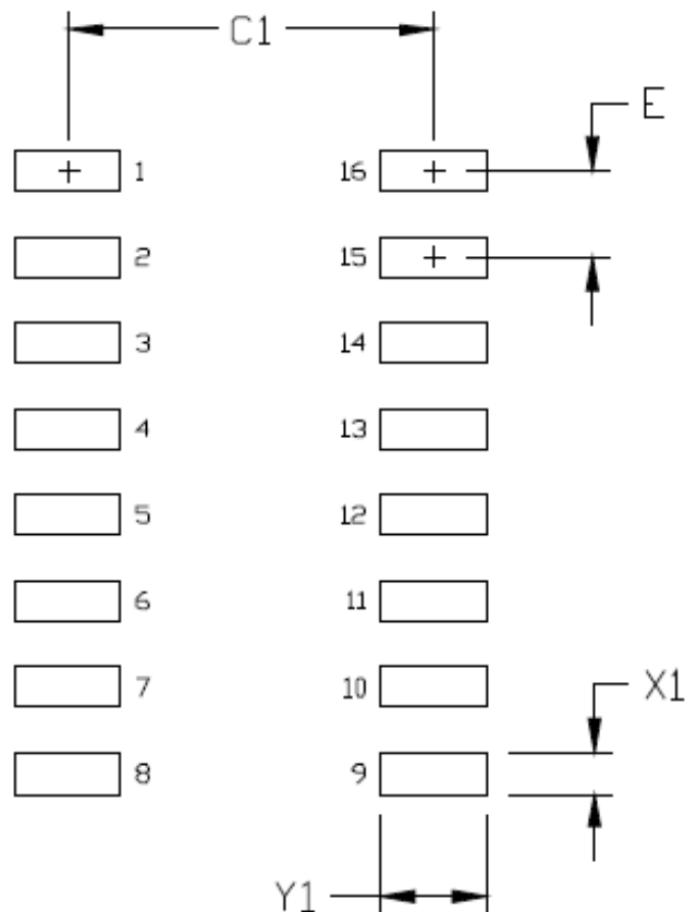
Figure 51. 16-Pin Narrow Body SOIC PCB Land Pattern
