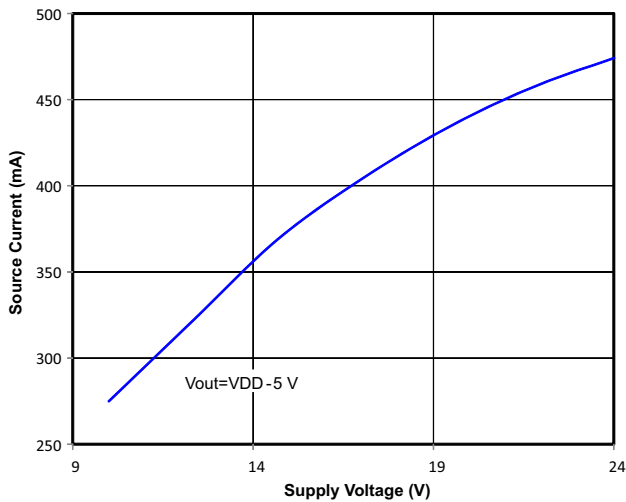
Figure 14. Output Source Current vs. Supply Voltage
