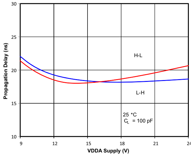
Figure 7. Propagation Delay vs. Supply Voltage
