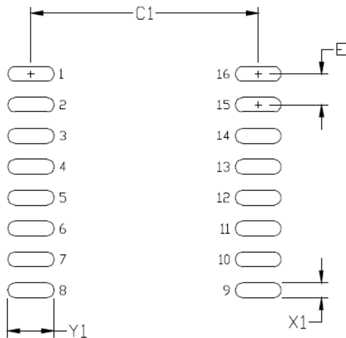
Figure 49. 16-Pin SOIC Land Pattern
