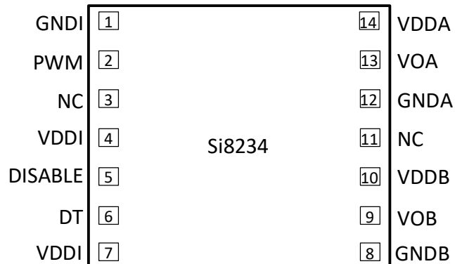
Figure 43. Si8234 LGA-14 (5x5 mm) Pinout
