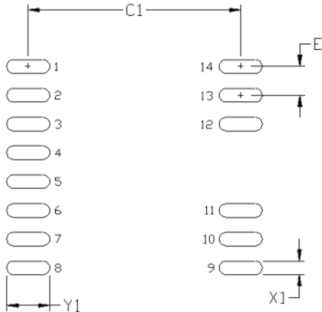
Figure 50. 14-Pin WB SOIC Land Pattern
