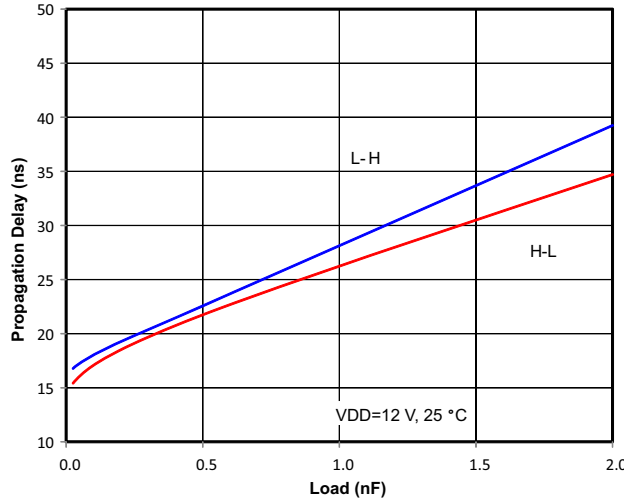
Figure 9. Propagation Delay vs. Load
