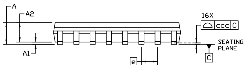
Figure 9.1. 16-Pin Narrow Body SOIC
