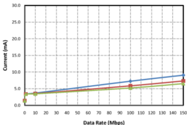
Figure 3.4. Si8641 Typical VDD1 Supply Current vs. Data Rate 5, 3.3, and 2.5 V Operation
