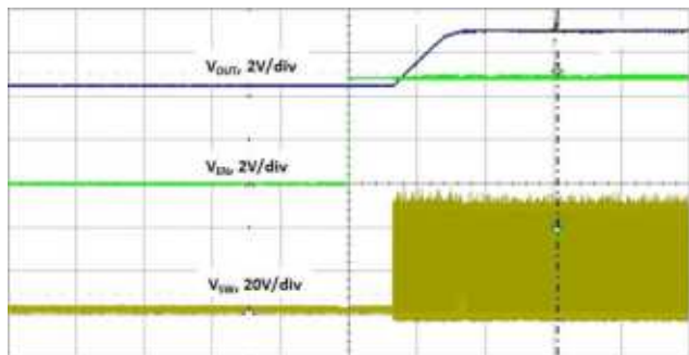
Fig. 8 - Pre-Bias Start-Up
