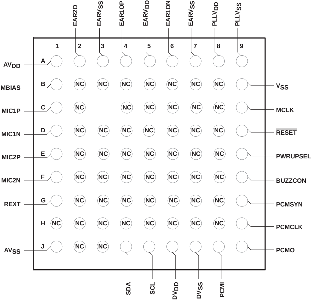
MicroStar Junior™ (GQE) PACKAGE (TOP VIEW)
