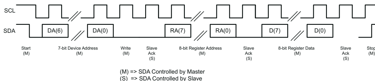
Figure 3-22. I²C Write
