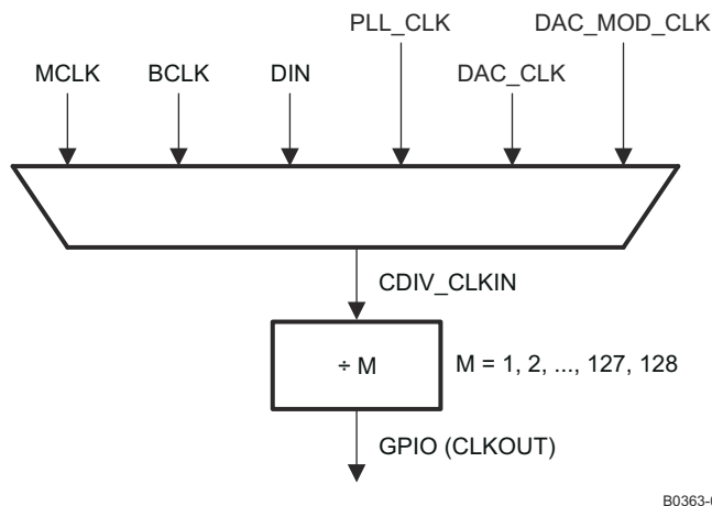
Figure 3-10. General-Purpose Clock Output Options
