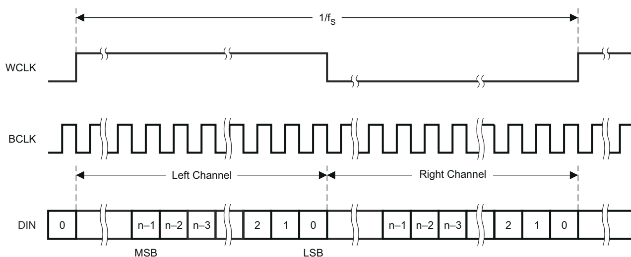
Figure 3-11. Timing Diagram for Right-Justified Mode
