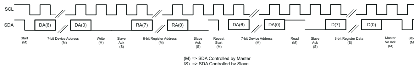
Figure 3-23. I²C Read
