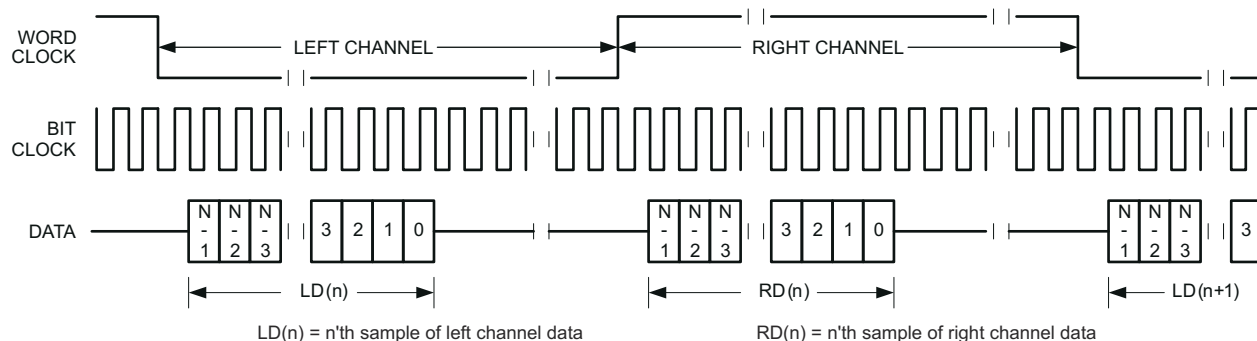
Figure 3-15. Timing Diagram for I 2 S Mode
