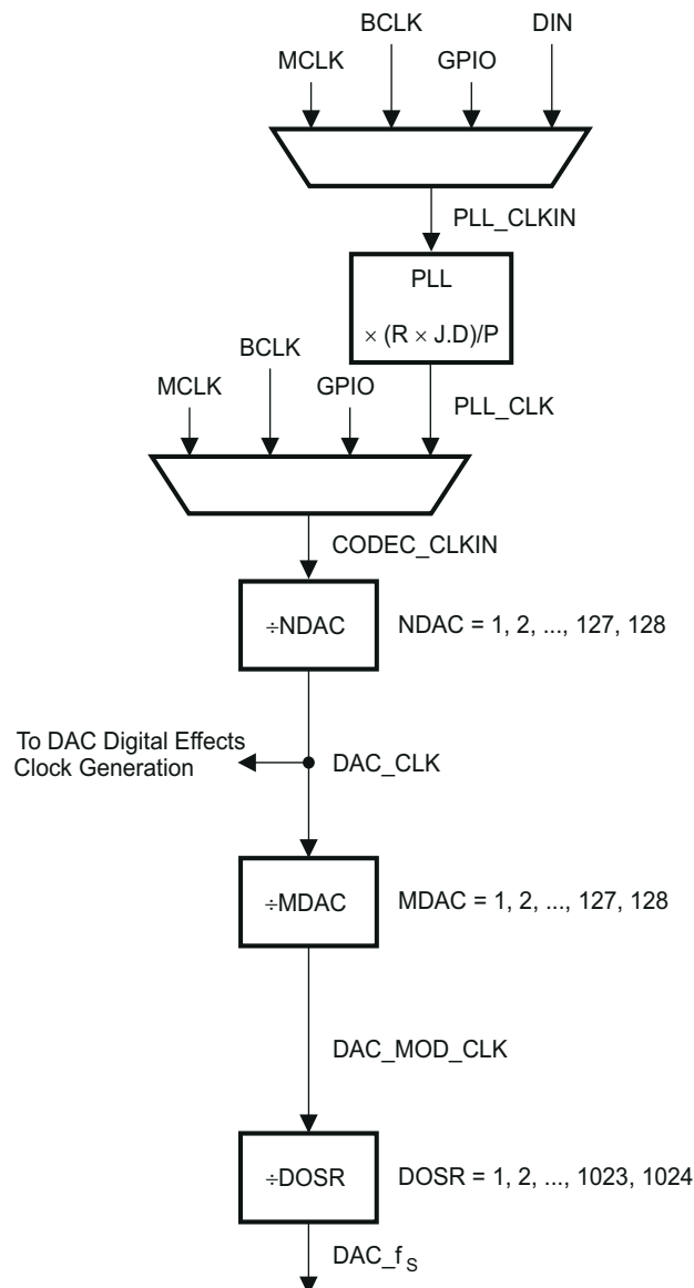
Figure 3-8. Clock Distribution Tree
