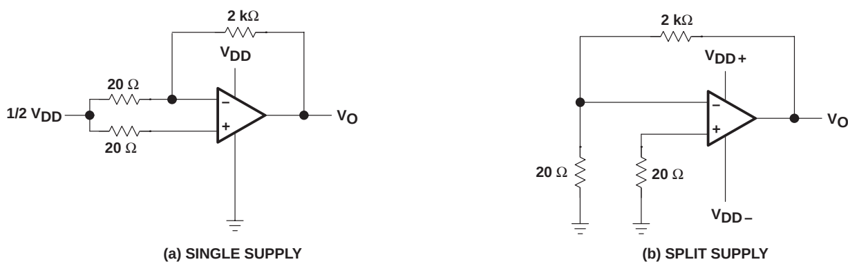
Figure 93. Noise-Test Circuits
