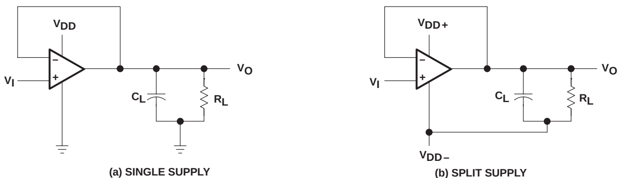
Figure 92. Unity-Gain Amplifier
