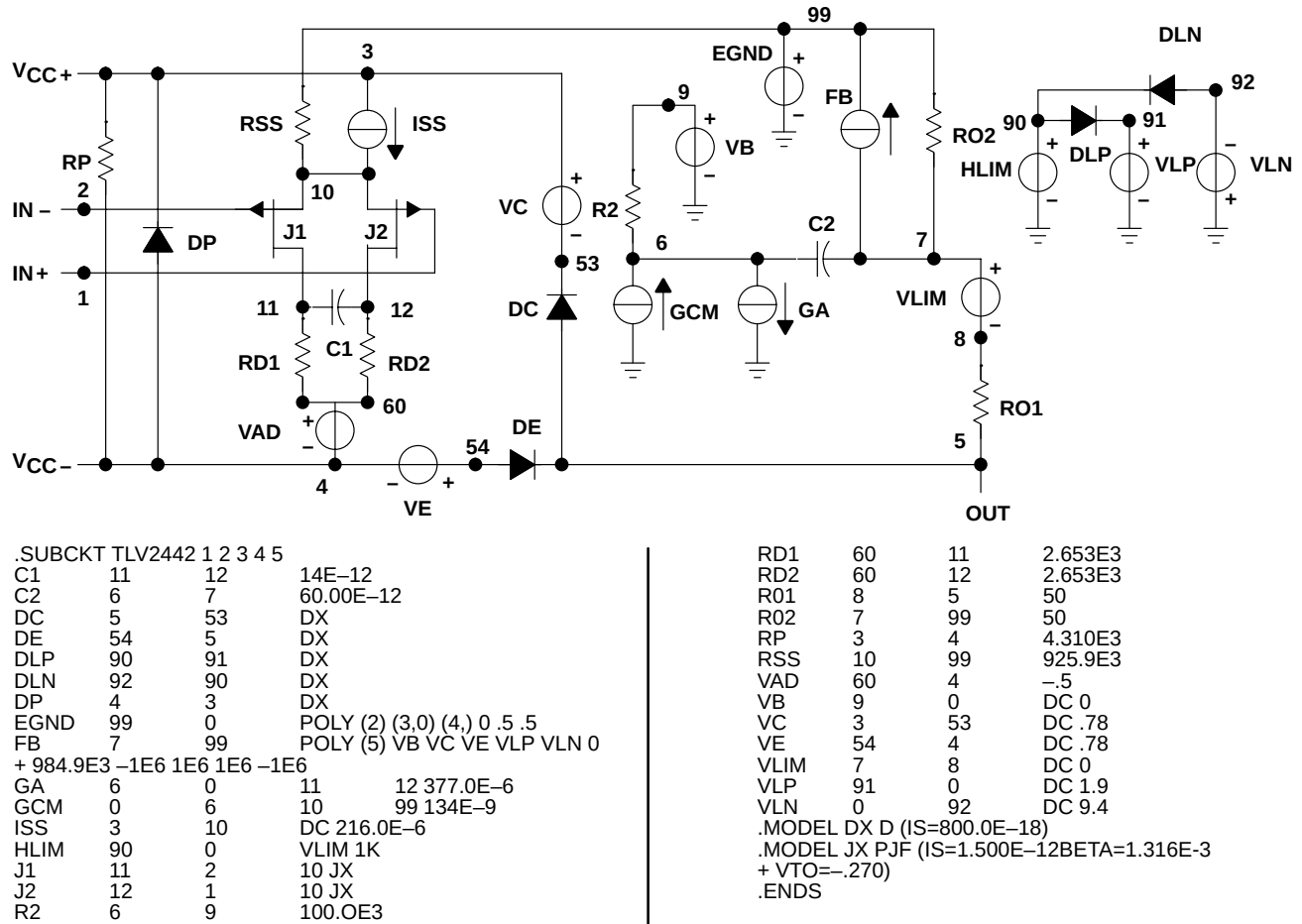
Figure 51. Boyle Macromodel and Subcircuit
