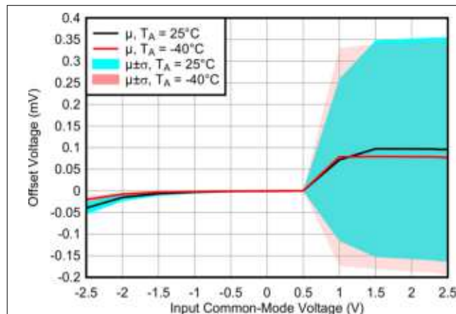
Figure 7-2. Offset Voltage vs Input Common-mode Voltage
