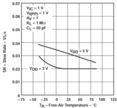
Figure 5-27. Slow Rate vs Free-Air Temperature
