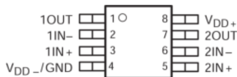
Figure 4-2. TLV2322 PW Package, 8-Pin TSSOP (Top View)
