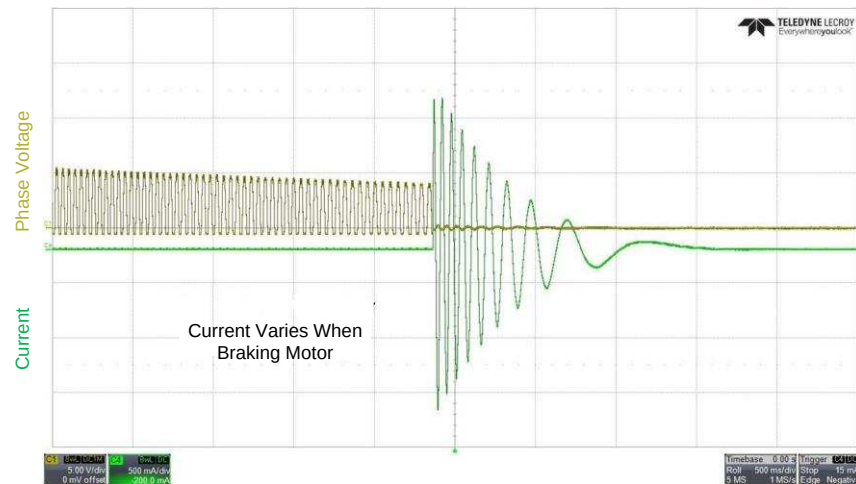
Figure 60. Brake Waveform
