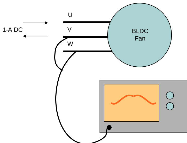
Figure 10. Oscilloscope Setup
