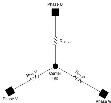
Figure 5. Wye-Connected Motor Resistance
