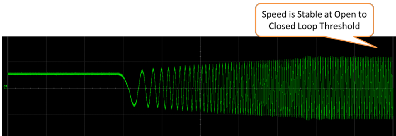
Figure 18. Speed Waveform
