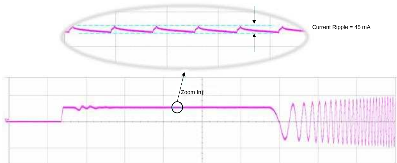
Figure 19. Ripple Amplitude
