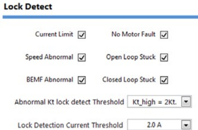
Figure 62. Lock Detect Settings
