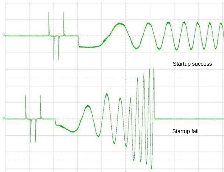
Figure 53. Startup Success versus Fail
