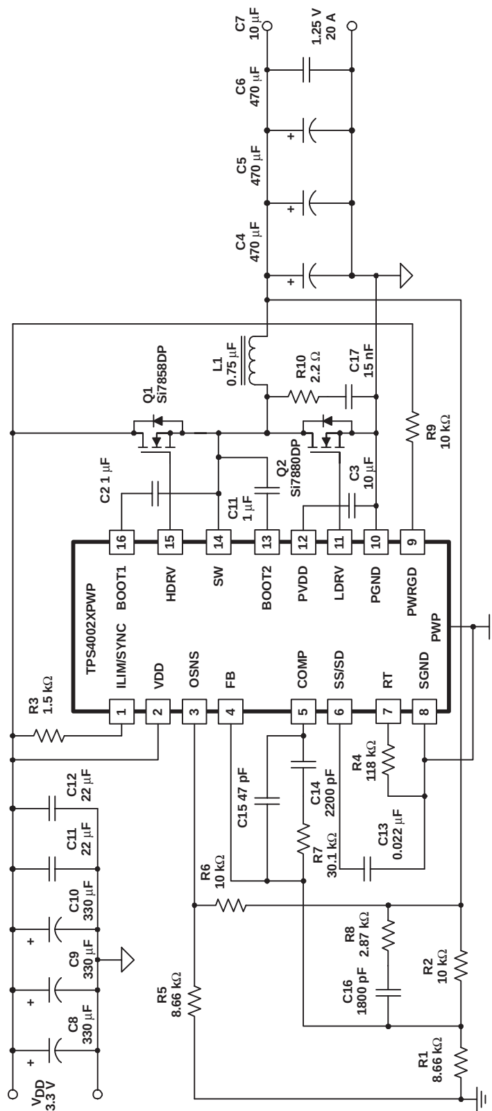
Figure 1. Typical Application
