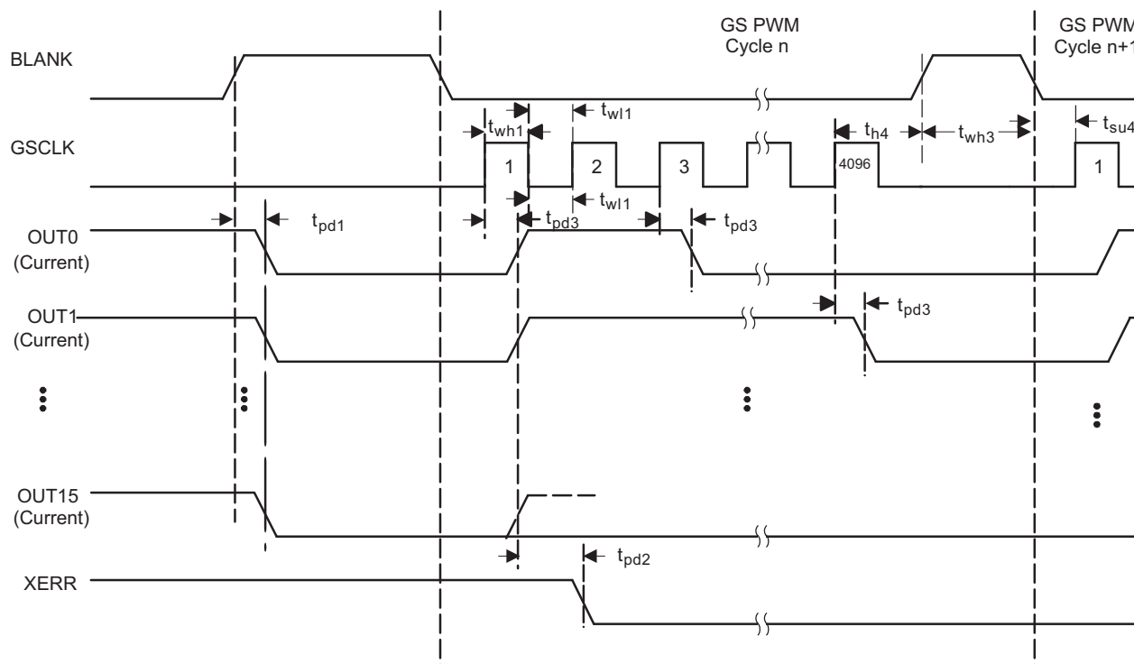
Figure 15. Grayscale PWM Cycle Timing Chart
