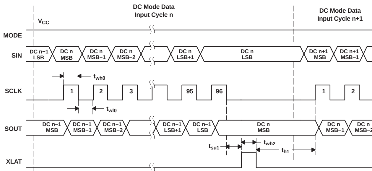
Figure 10. Dot Correction Data Input Timing Chart
