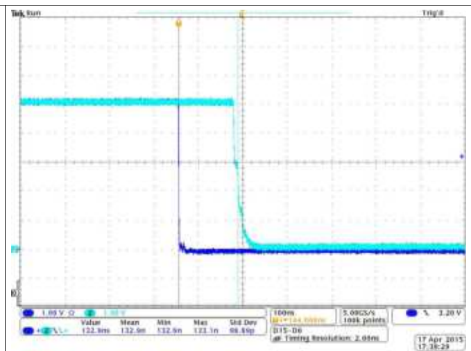
Figure 25. t_{\text{LOOP}} Delay Waveform Recessive to Dominant
