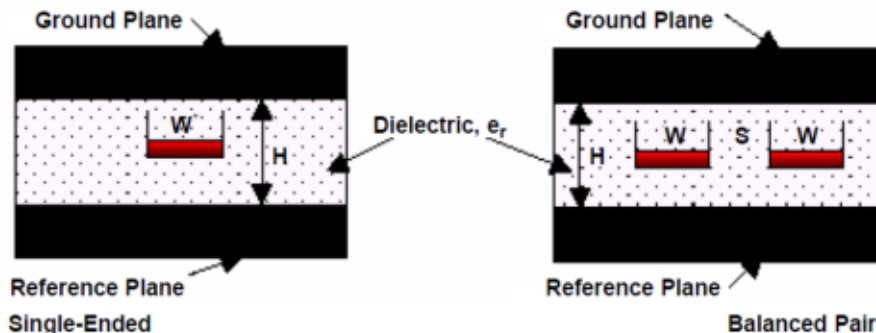
Figure 22. Stripline Topology
