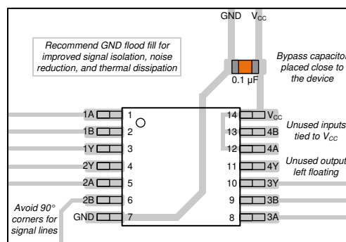
Figure 8-3. Example Layout for the SN74HCS266-Q1
