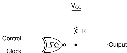
Figure 8-1. Typical application block diagram
