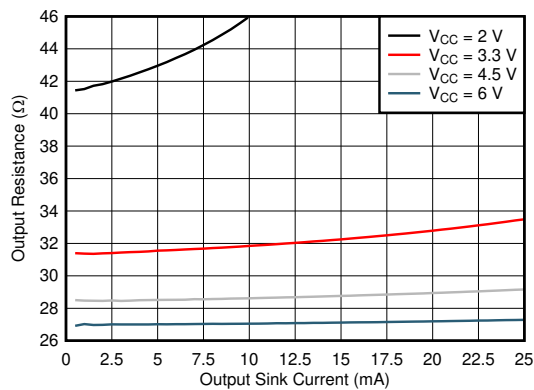
Figure 5-1. Output Driver Resistance in Low State
