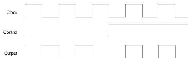
Figure 8-2. Application timing diagram
