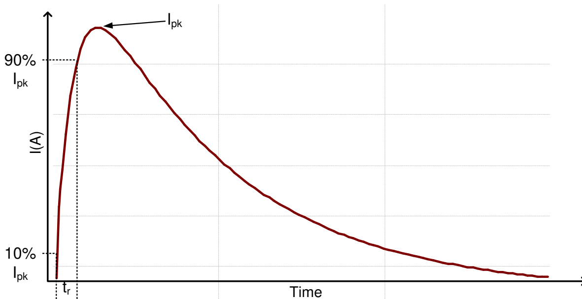
Figure 10-2. HBM Curve
