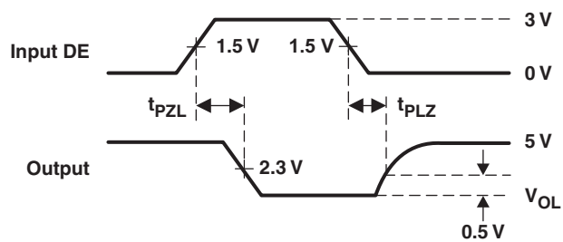
VOLTAGE WAVEFORMS
