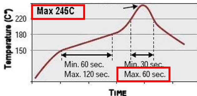
RECOMMENDED TEMPERATURE PROFILE FOR SN-AG-CU Pb-FREE SOLDER PASTE
