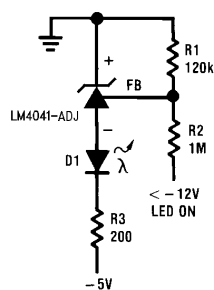
Figure 8-6. Voltage Level Detector
