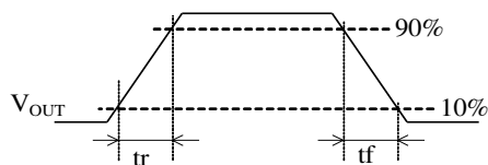
Figure 2 Switching time
