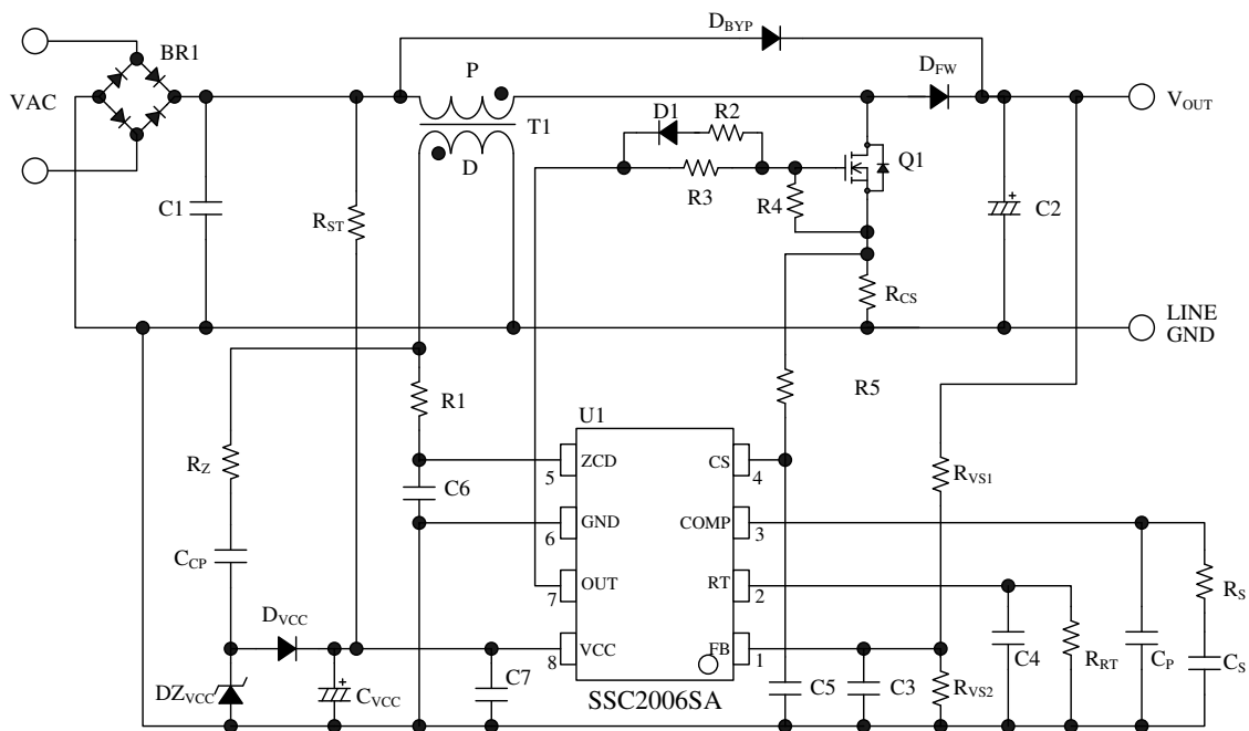
Figure 5-2 Power supply from an auxiliary winding
