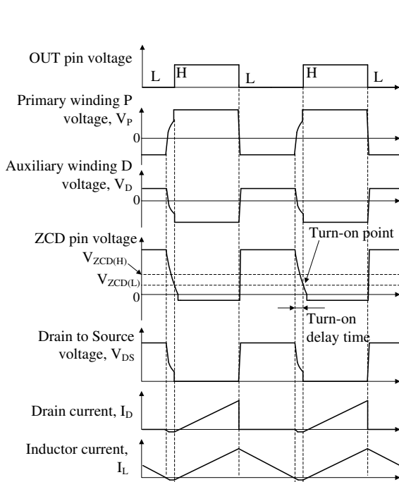
Figure 8-11 Zero current detection waveform
