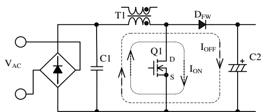
Figure 8-1 PFC circuit
