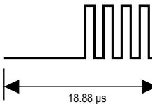
Figure 85. Logic 1, high data rate, fast commands
