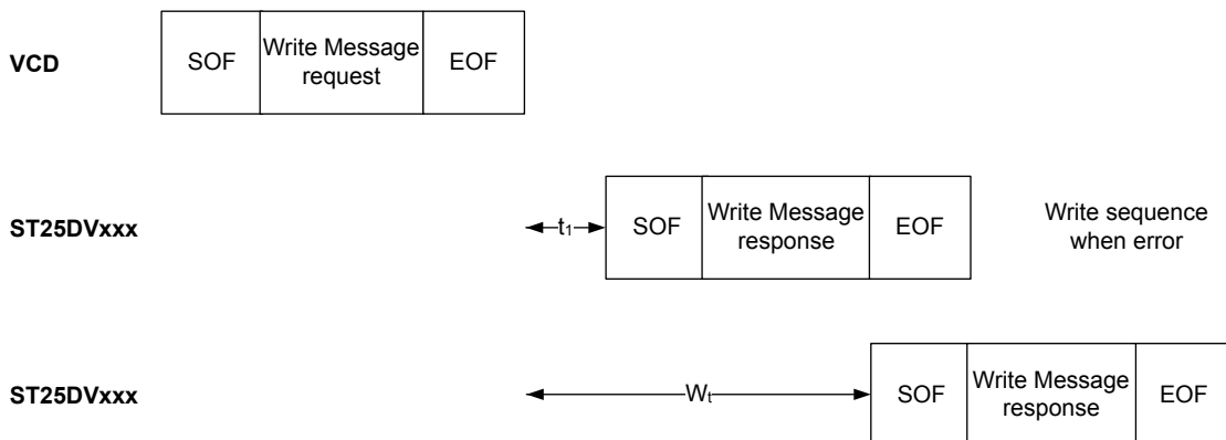
Figure 59. Manage GPO frame exchange between VCD and ST25DVxxx
