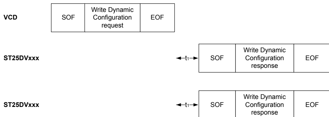
Figure 58. Write Dynamic Configuration frame exchange between VCD and ST25DVxxx
