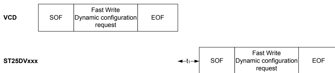
Figure 73. Fast Write Dynamic Configuration frame exchange between VCD and ST25DVxxx
