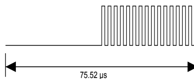
Figure 87. Logic 1, low data rate, fast commands
