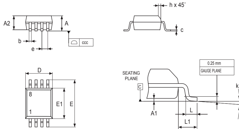
Figure 84. SO8N - Outline
