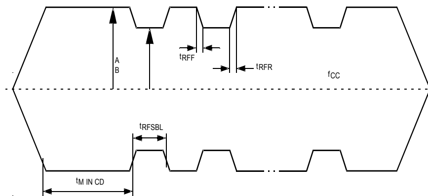
Figure 83. ASK modulated signal
