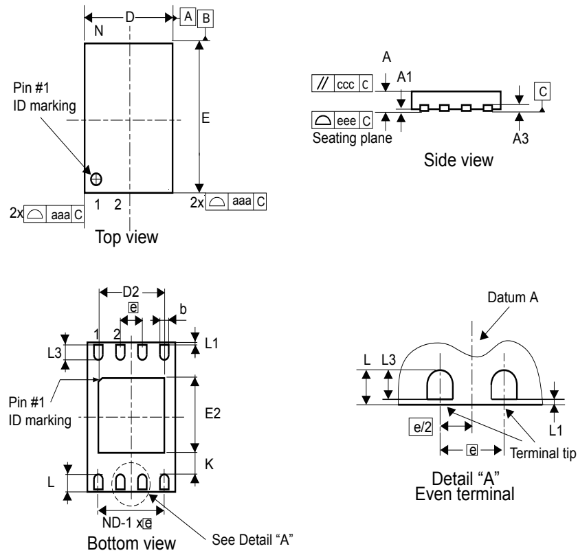
Figure 88. UDFN8 - Outline
