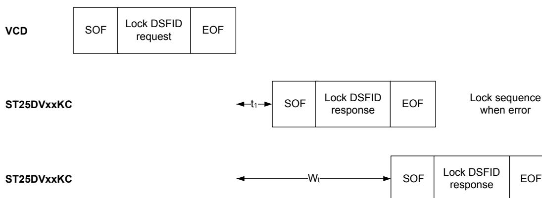
Figure 56. Lock DSFID frame exchange
