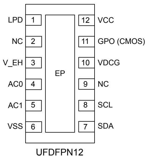
Figure 6. UDFPN12 package connections
