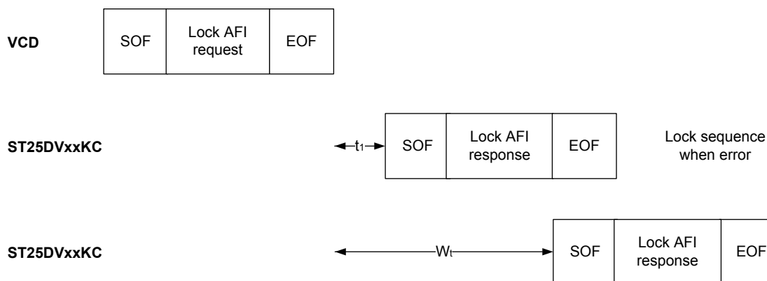
Figure 54. Lock AFI frame exchange
