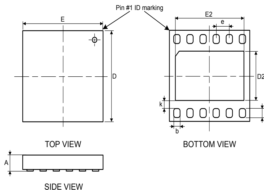
Figure 91. UFDFPN12 - Outline
