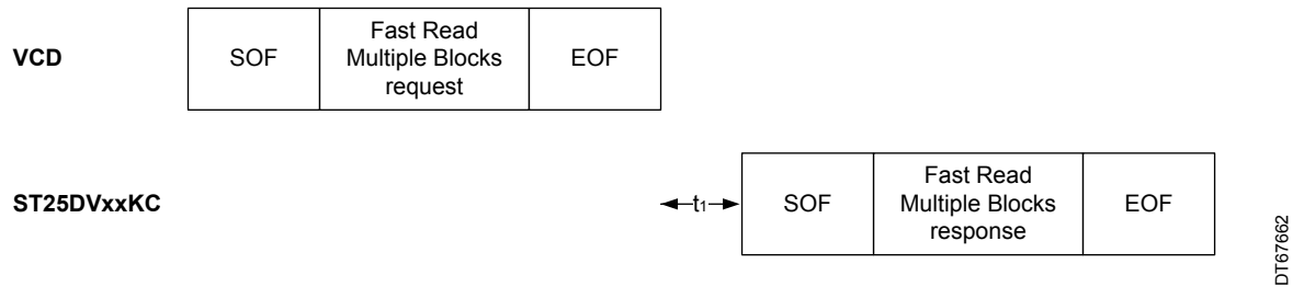
Figure 74. Fast Read Multiple Blocks frame exchange
