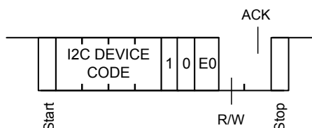
Figure 15. RFSwitchOff command
