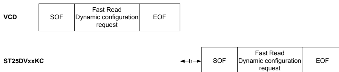
Figure 78. Fast Read Dynamic Configuration frame exchange
