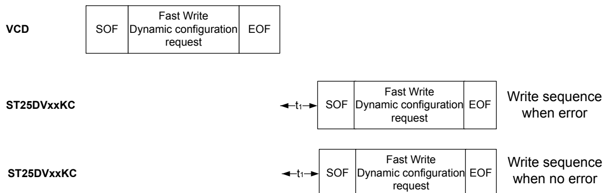
Figure 79. Fast Write Dynamic Configuration frame exchange
