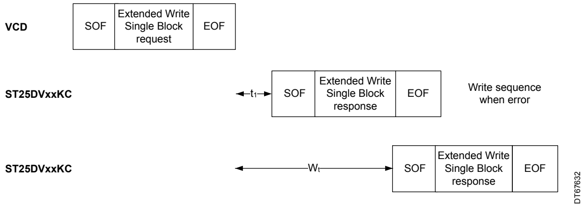
Figure 44. Extended Write Single Block frame exchange
