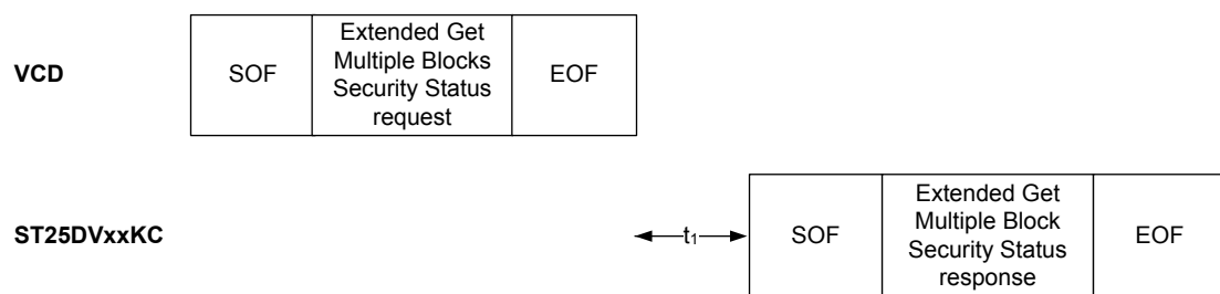
Figure 60. Extended Get Multiple Blocks Security Status frame exchange
