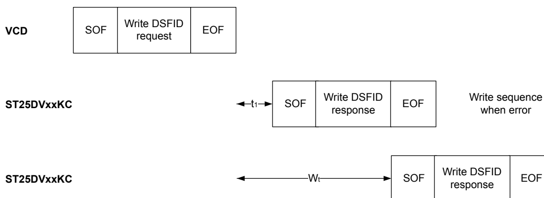
Figure 55. Write DSFID frame exchange
