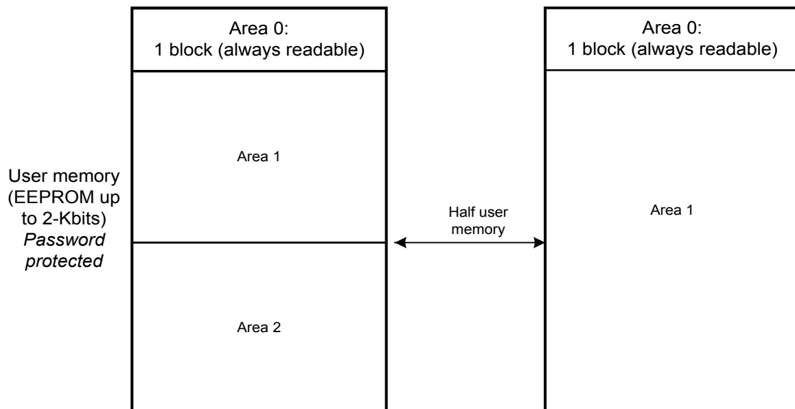
Figure 5. Memory organization
