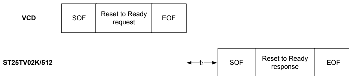
Figure 16. Reset to Ready frame exchange between VCD and ST25TV02K/512
