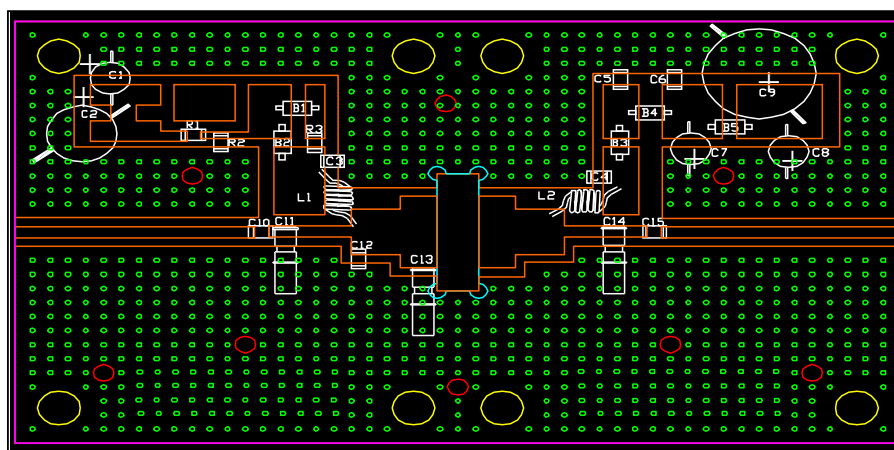
Figure 11. Circuit layout
