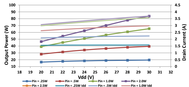
Figure 5. Output power and drain current vs V_{DD} and input power ( I_{dq} = 300 mA, f_o = 945 MHz tuned at V_{DD} = 28 V)
