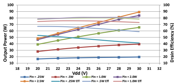
Figure 4. Output power and efficiency vs V_{DD} and input power ( I_{dq} = 300 mA, f_o = 945 MHz tuned at V_{DD} = 28 V)
