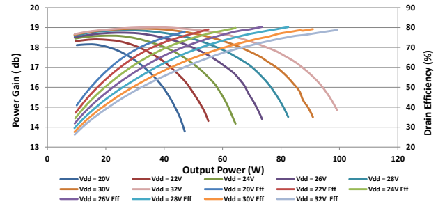
Figure 3. Power gain and efficiency vs output power and V_{DD} ( I_{dq} = 300 mA, f_o = 945 MHz tuned at V_{DD} = 28 V)
