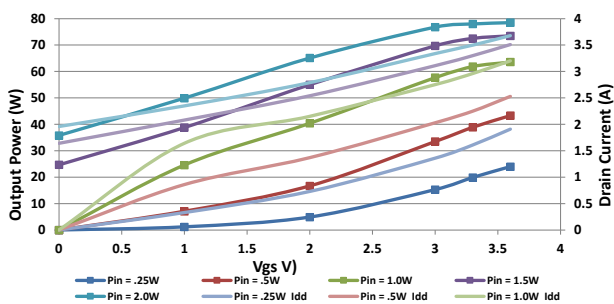
Figure 6. Output power and drain current vs V_{GS} and input power ( V_{DD} = 28 V, f_o = 945 MHz)
