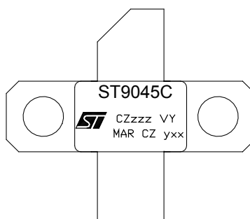
Figure 13. Marking layout
