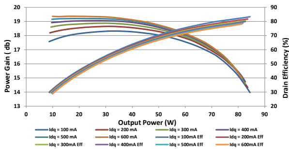
Figure 2. Power gain and efficiency vs output power and I_{dq} ( V_{DD} = 28 V, f_o = 945 MHz)
