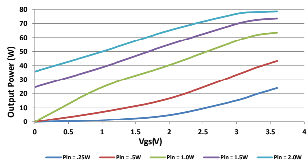
Figure 7. Output power vs V_{GS} and input power ( V_{DD} = 28 V, f_o = 945 MHz)
