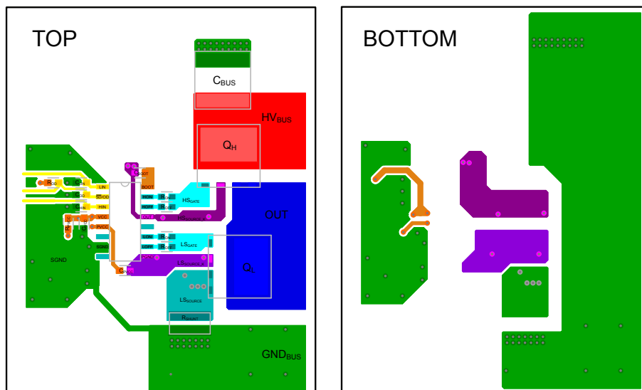
Figure 13. Two-layer layout example
