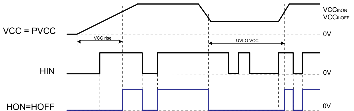
Figure 4. VCC UVLO and HON, HOFF
