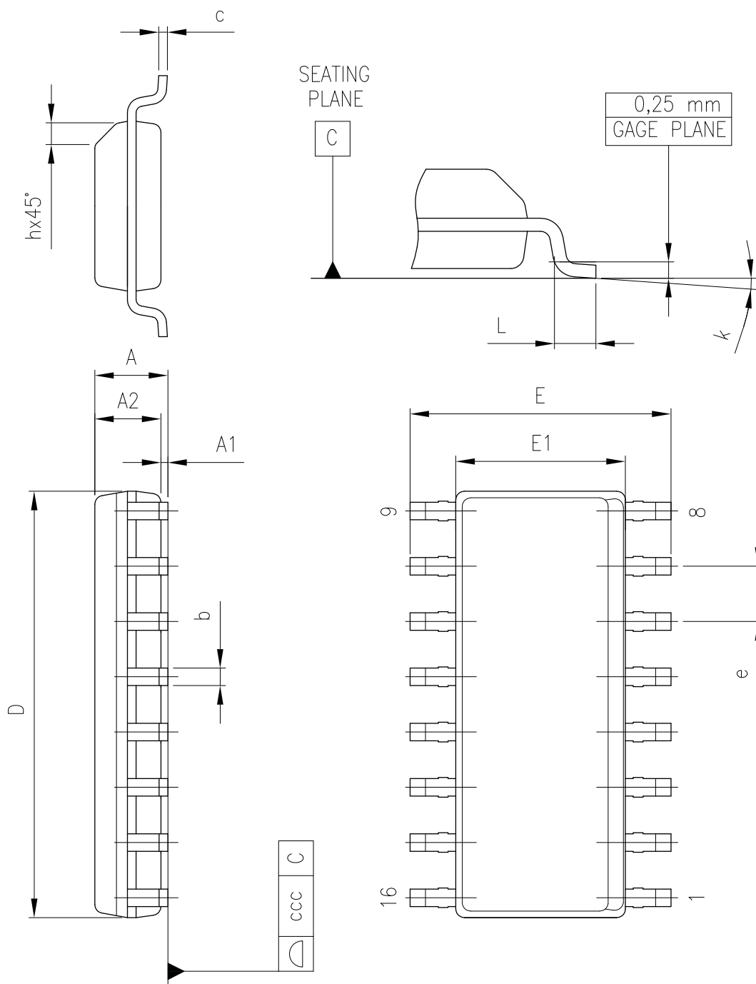
Figure 16. SO-16 mechanical data
