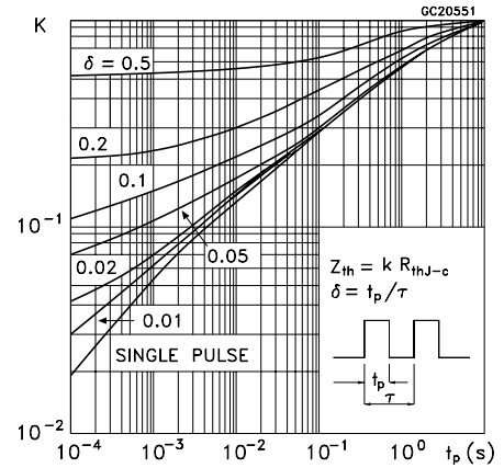
Figure 2. Thermal impedance
