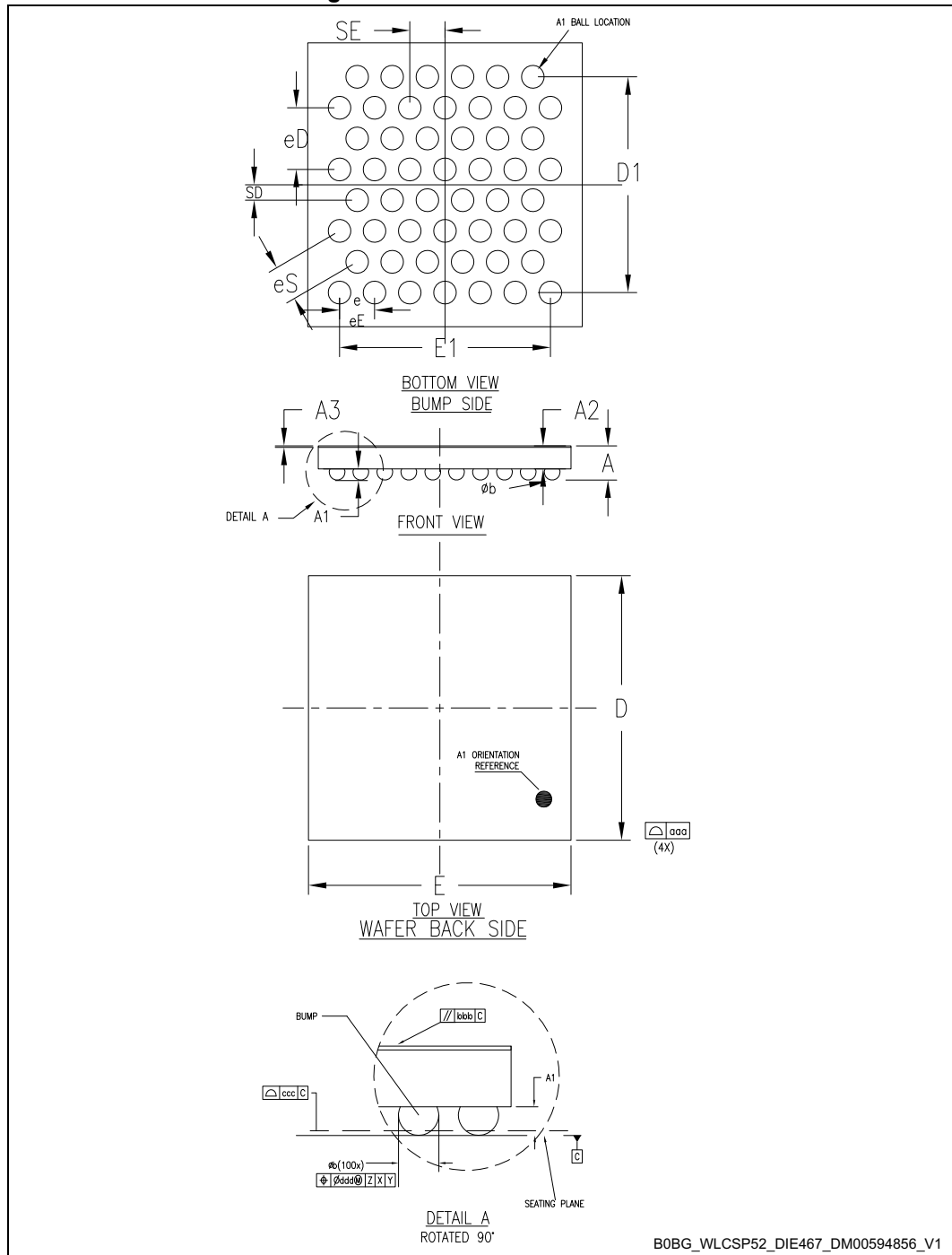
Figure 47. WLCSP52 - Outline
