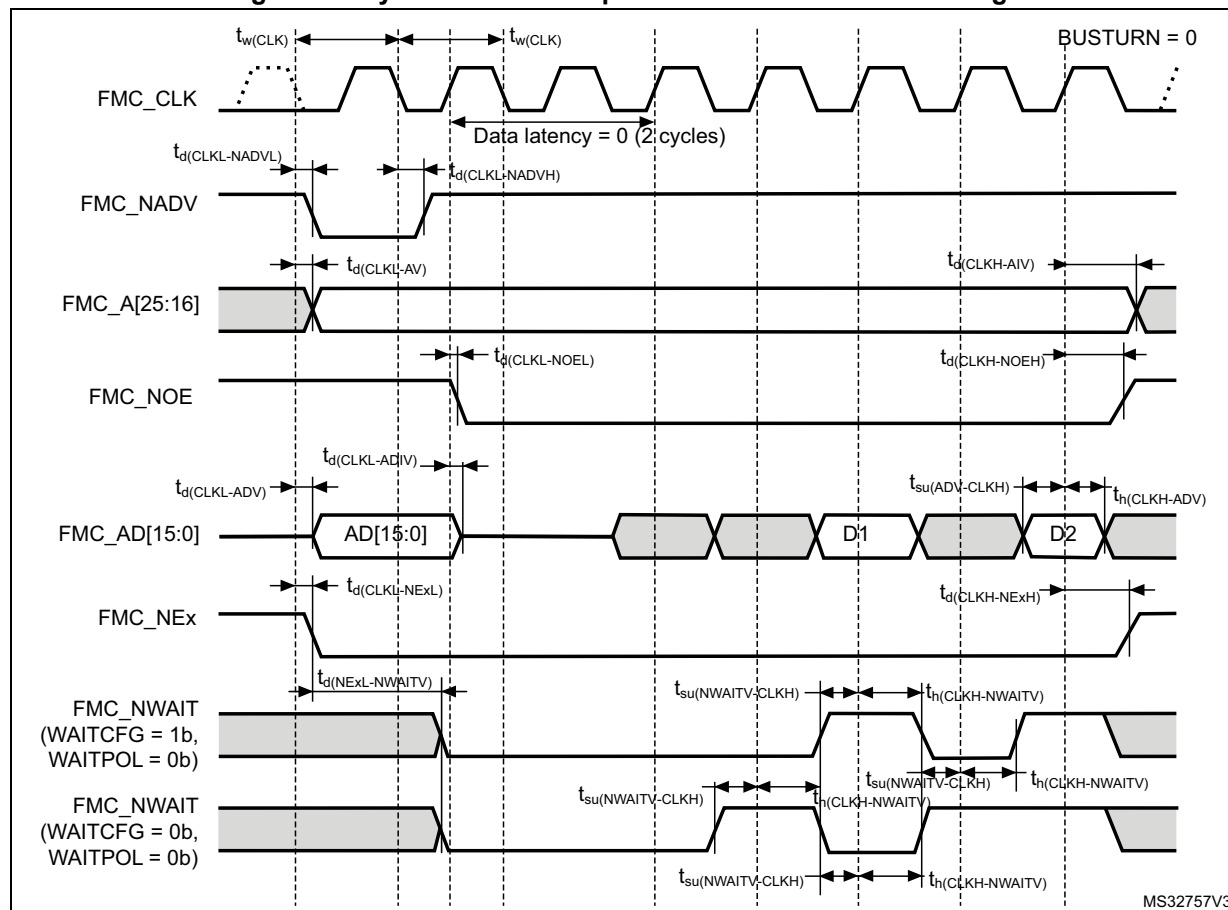
Figure 29. Synchronous multiplexed NOR/PSRAM read timings
