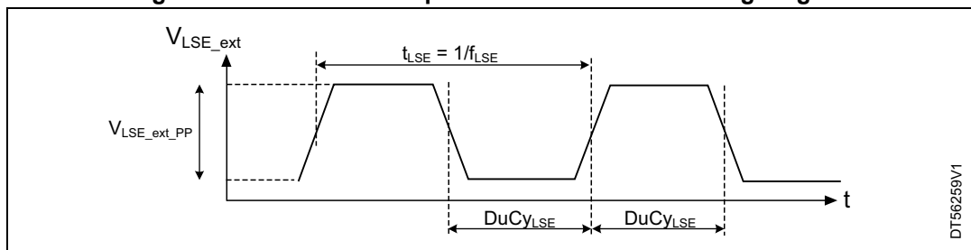
Figure 20. LSE external square clock source AC timing diagram
