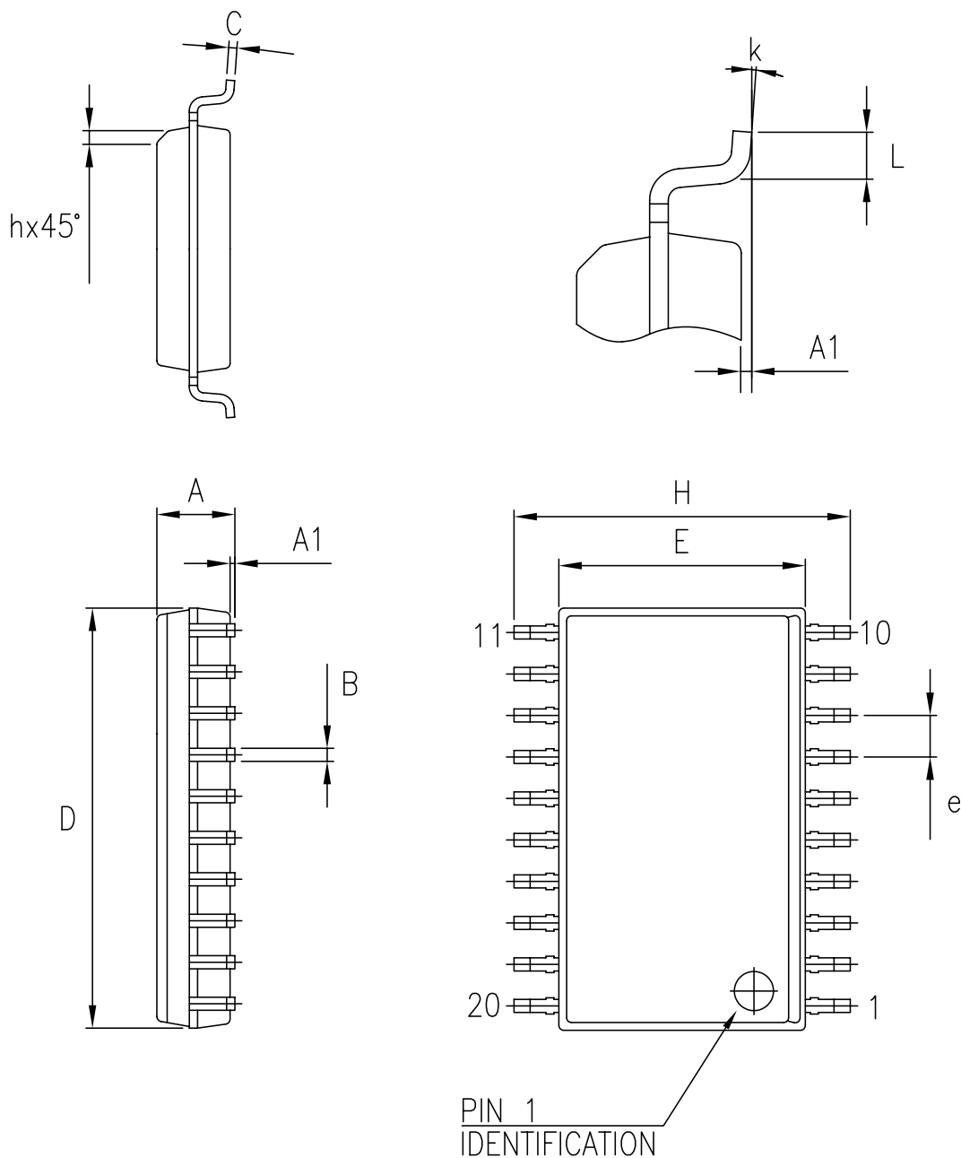
Figure 5. SO20 package outline
