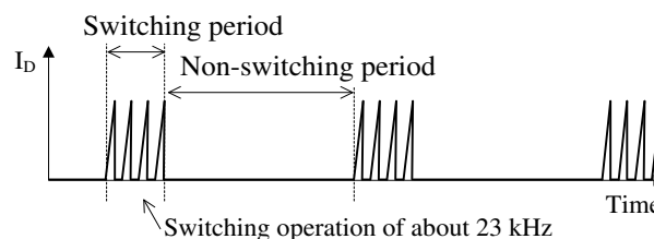
Figure 10-13. Switching Waveform at Burst Oscillation Mode
