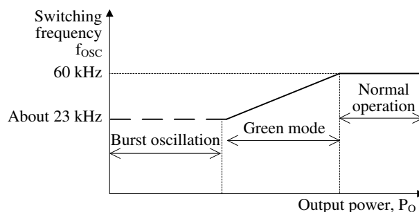
Figure 10-12. Switching Frequency in Response to P_o
