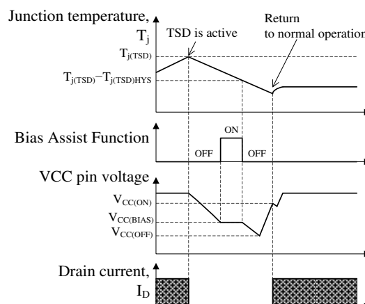
Figure 10-17. TSD Operational Waveforms
