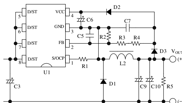
Figure 11-1. Peripheral Circuit of IC in Buck Converter
