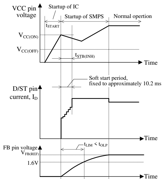
Figure 10-3. Startup Waveforms
