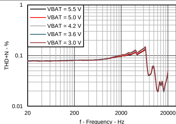
Figure 53. THD+N vs Frequency (8Ω) for Digital Input
