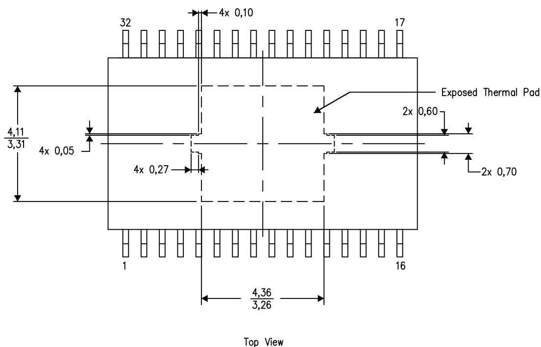
Exposed Thermal Pad Dimensions
