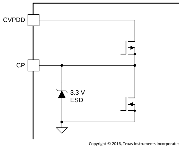
Figure 13. CP Pin
