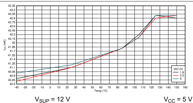
Figure 11-9. Normal Mode: I_{CC} vs Temperature Dominant
