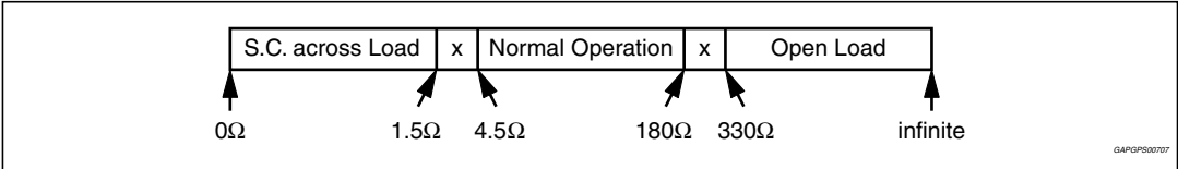
Figure 28. Load detection thresholds - high gain setting
