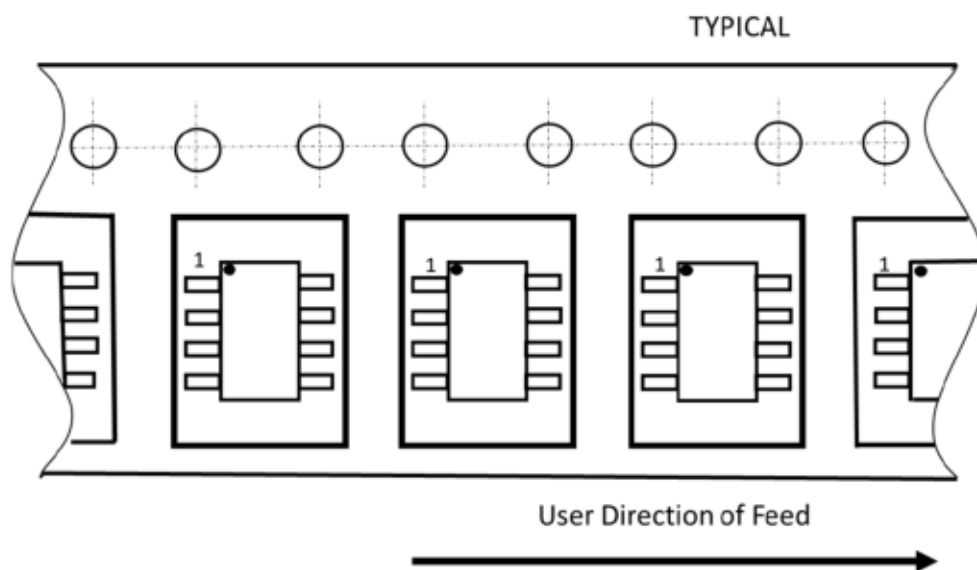
Figure 10. Tape orientation
