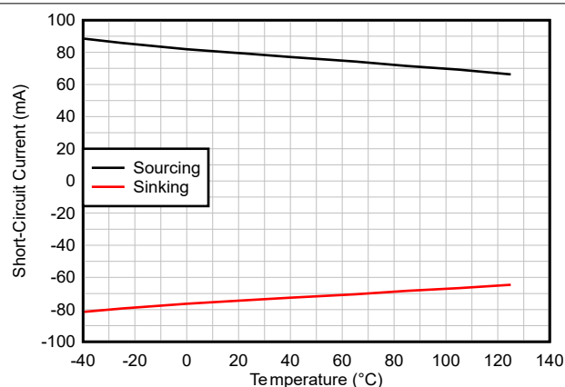
Figure 5-7. Short-Circuit Current vs Temperature
