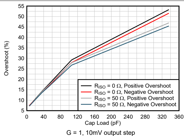
Figure 5-11. Small-Signal Overshoot vs Capacitive Load
