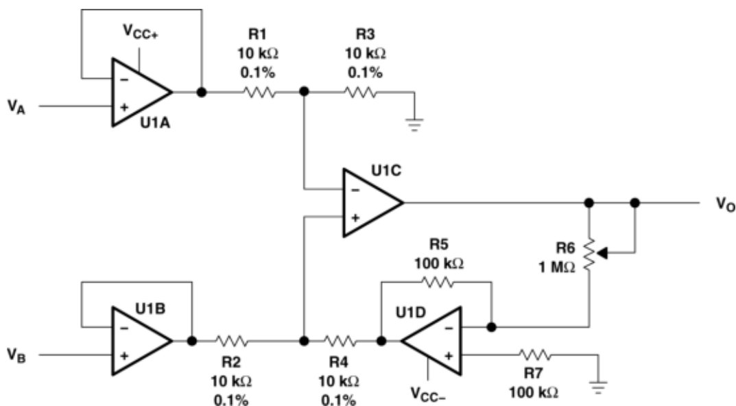
Figure 7-7. Instrumentation Amplifier with Linear Gain-Adjust Circuit
