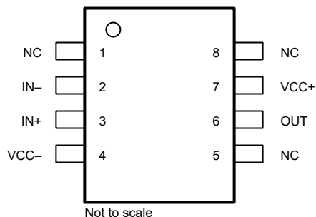
Figure 4-2. TL031x, TL031Ax D or P Package, 8-Pin SOIC or PDIP (Top View)
