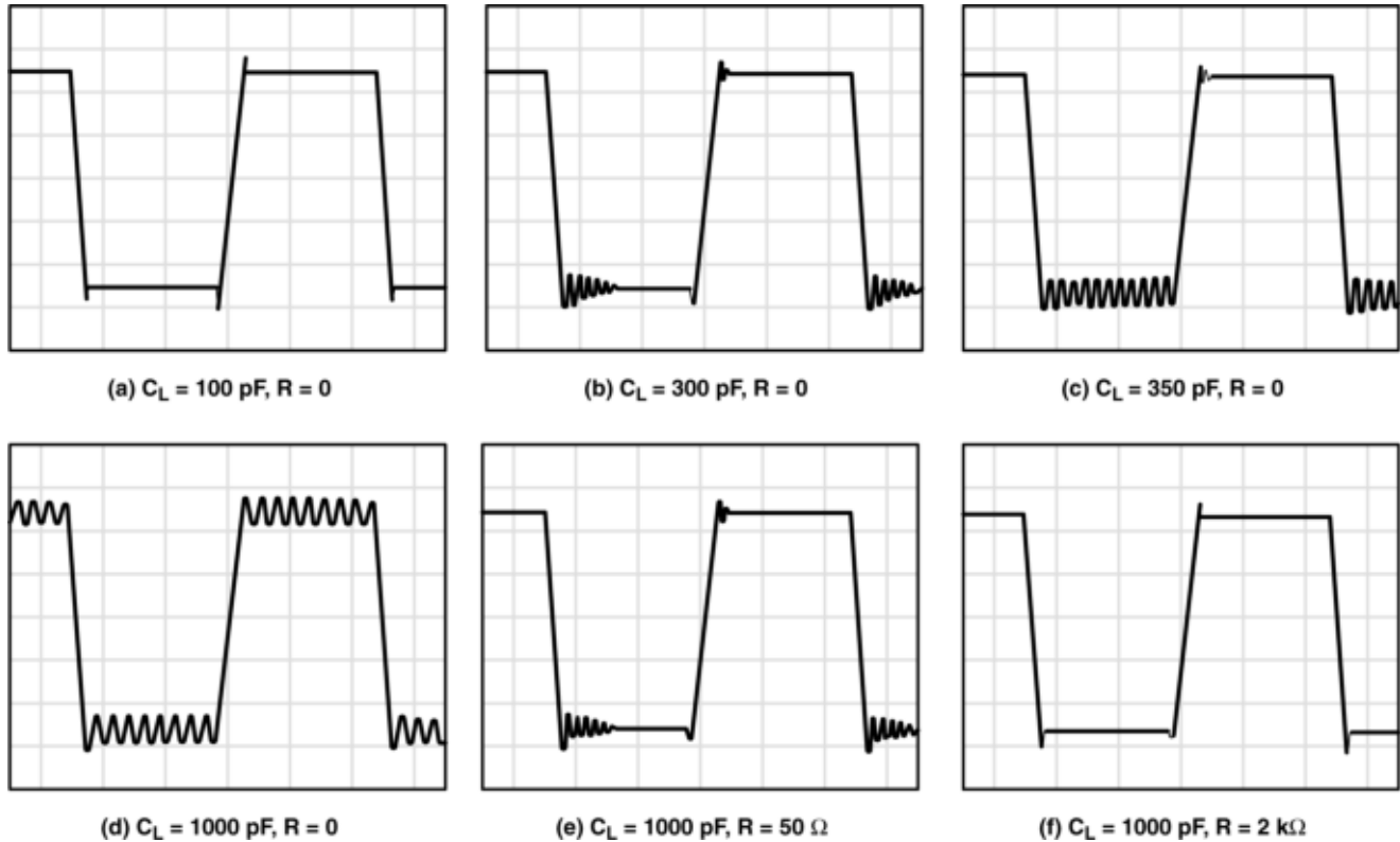
Figure 7-2. Effect of Capacitive Loads
