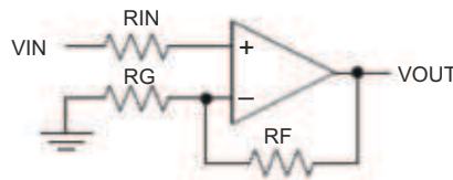
Figure 8-5. Schematic Representation
