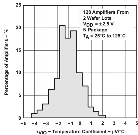
Figure 6-9. Distribution of TLC2274-Q1 vs Input Offset Voltage Temperature Coefficient
