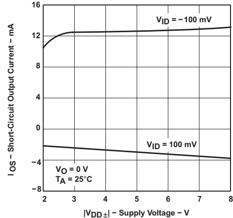
Figure 6-20. Short-Circuit Output Current vs Supply Voltage
