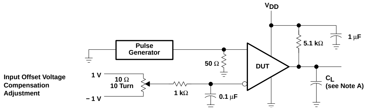
TEST CIRCUIT
