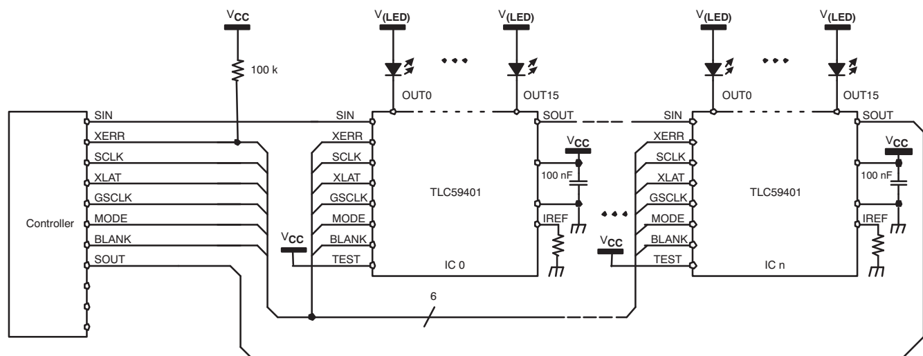
Figure 22. Cascading Devices
