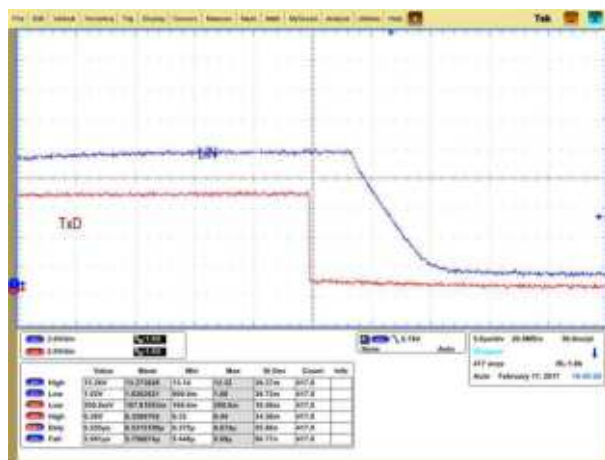
Figure 9-2. Recessive to Dominant Propagation
