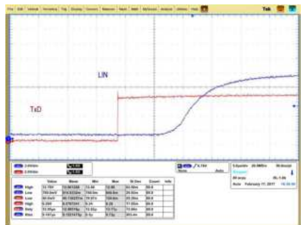
Figure 9-3. Dominant to Recessive Propagation
