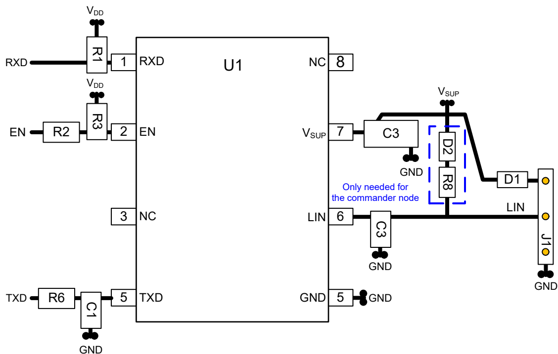
Figure 11-1. Layout Example
