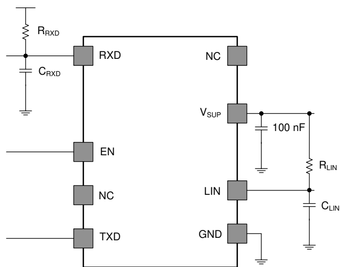
Figure 7-17. Wake-up through LIN
