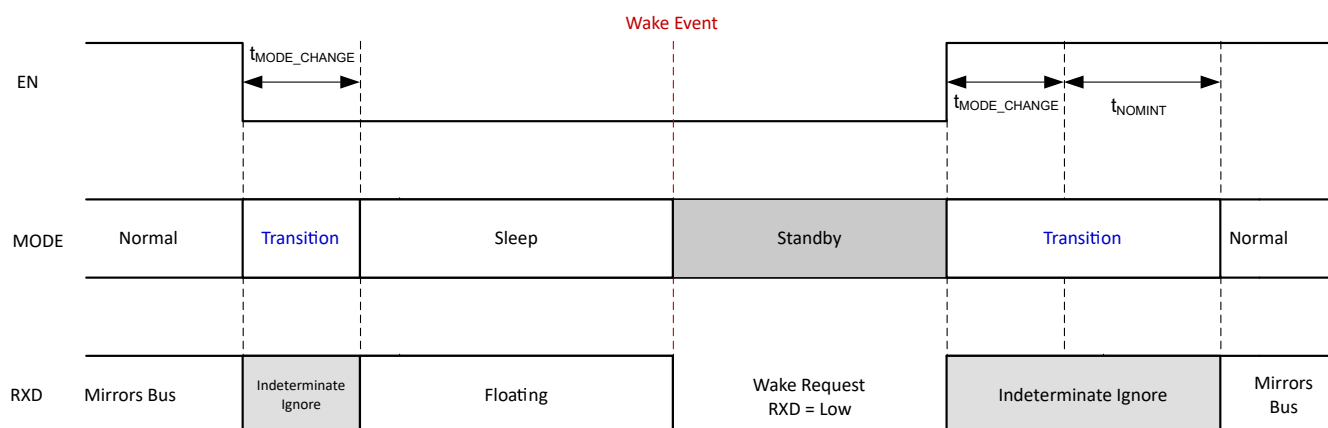
Figure 7-15. Mode Transitions
